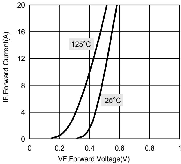
Fig1. Typical Forward Current and Forward Voltage
